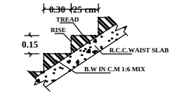
SECTION OF STAIRCASE
