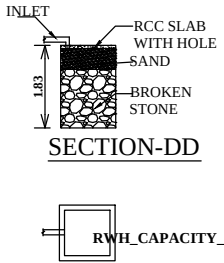
PLAN OF RWH
