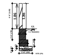
COMPOUND WALL
