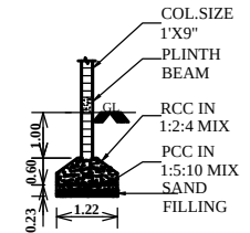
COLUMN DETAILS
