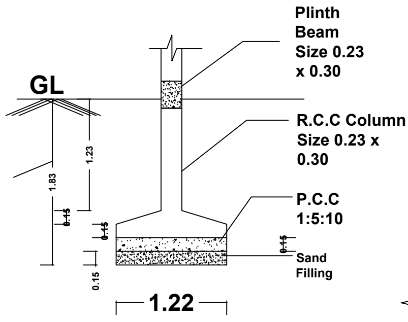
FOUNDATION DETAILS
