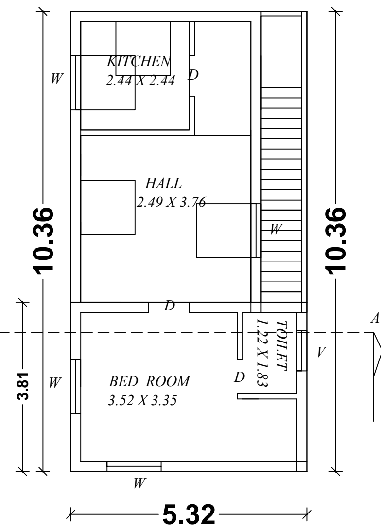
EXG.FIRST FLOOR AND EXTN.FIRST FLOOR PLAN
