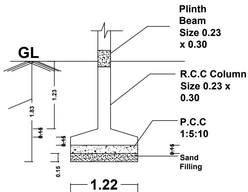
FOUNDATION DETAILS
