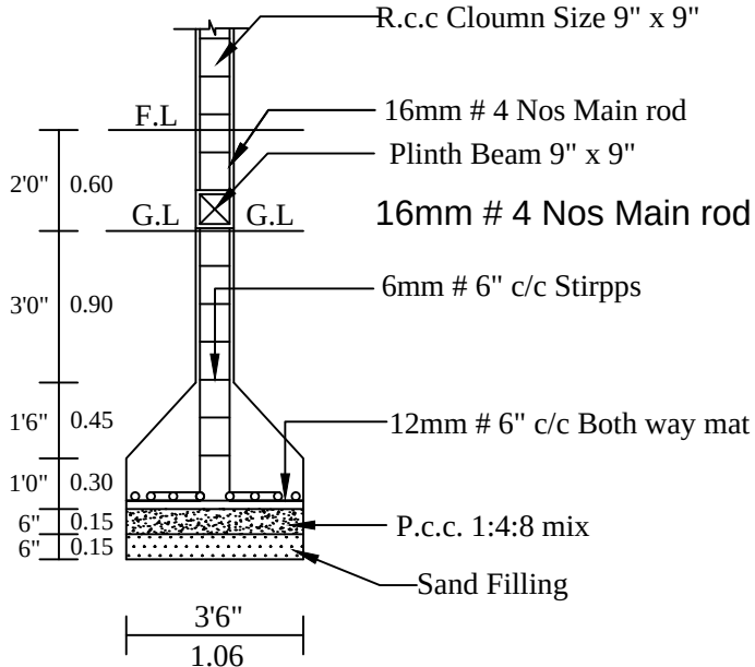
COLUMN DETIAL
