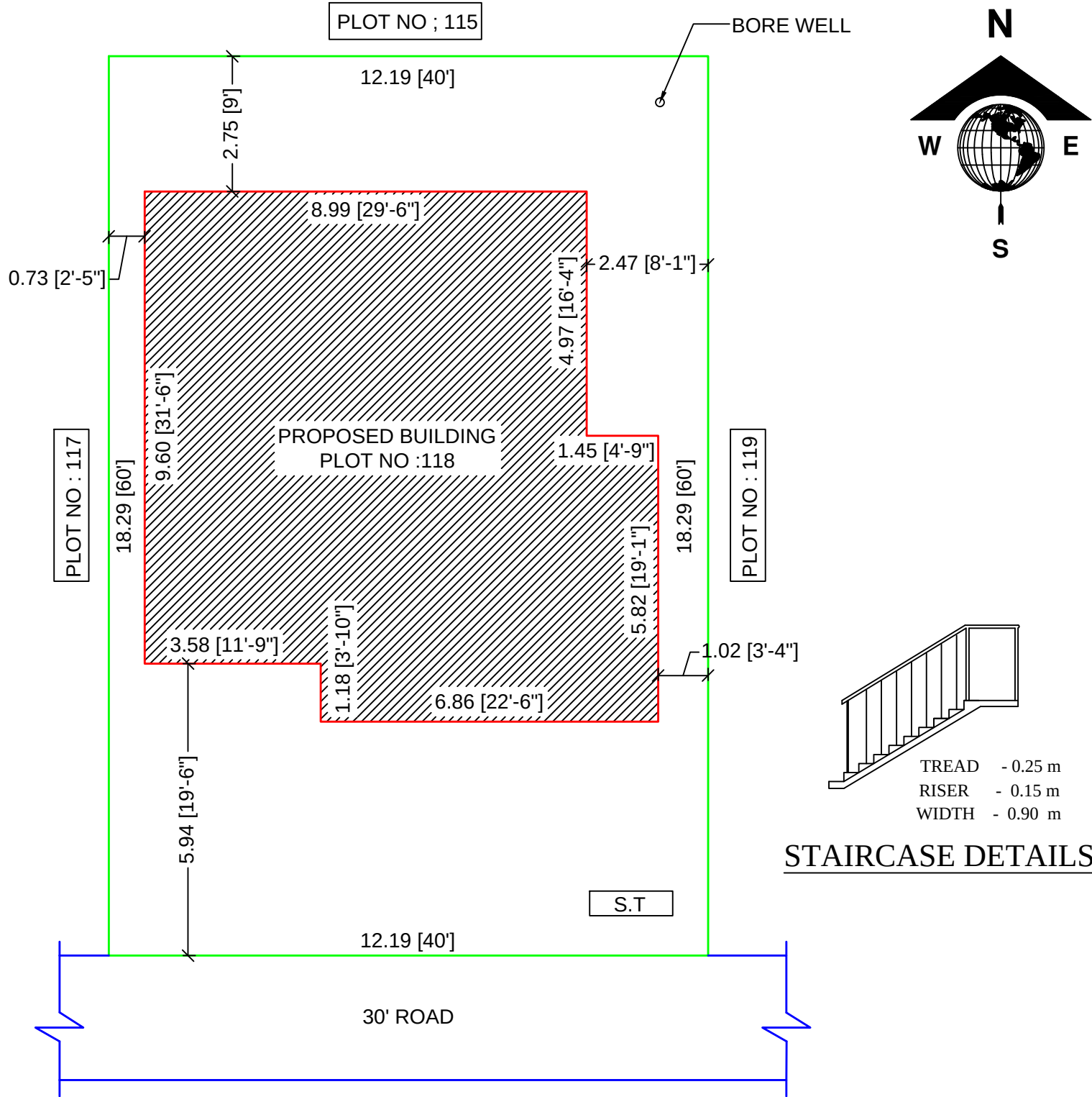
SITE PLAN (1:100)
