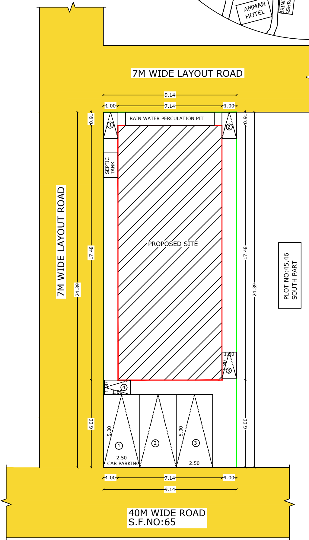
SITE PLAN
