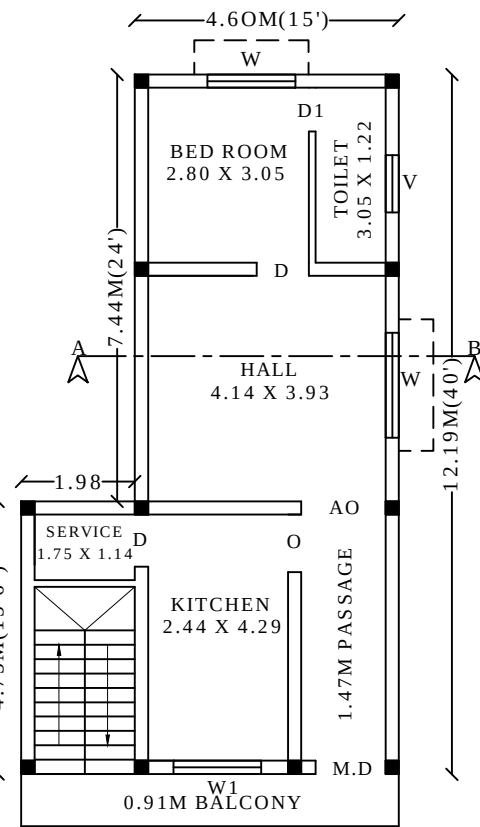
PRO.GROUND FLOOR PLAN (EAST FACING)
