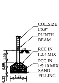
COLUMN DETAILS
