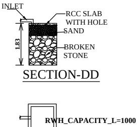
PLAN OF RWH
