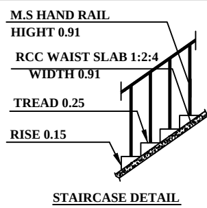
STAIRCASE DETAIL
