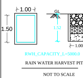
RAIN WATER HARVEST PIT
