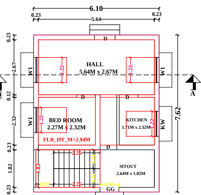
FLOOR-0 PRO.GROUND FLOOR PLAN
