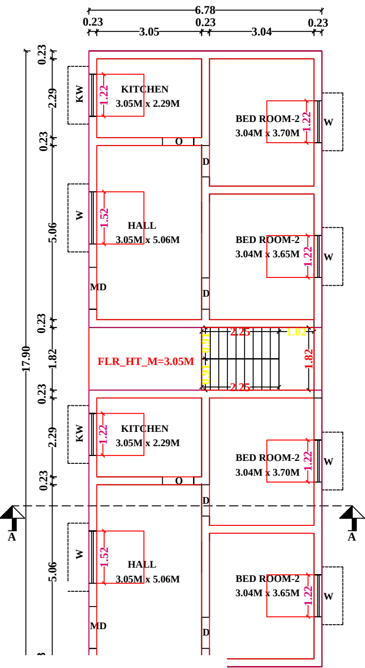
R-0 FLOOR PLAN
