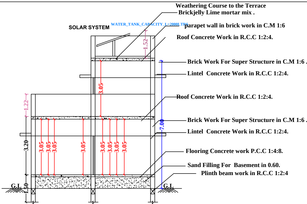
SECTION-AB
