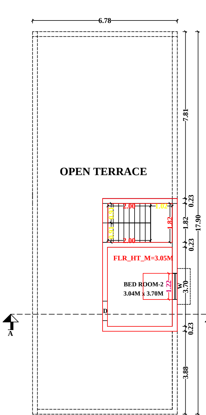
FLOOR-1 PRO.FIRST FLOOR PLAN
