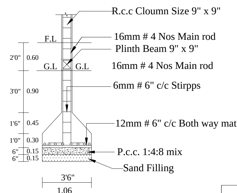
COLUMN DETIAL
