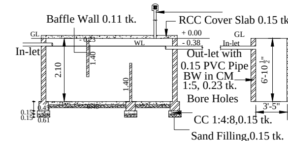
SEPTIC TANK & SOAK PIT
