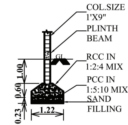
COLUMN DETAILS
