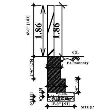
COMPOUND WALL
