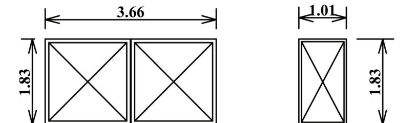
MAIN GATE
