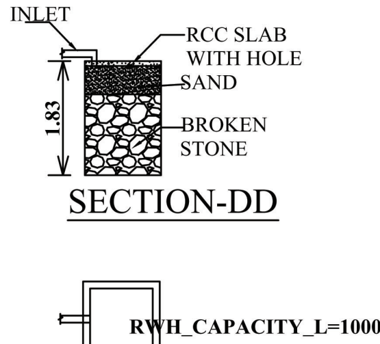
PLAN OF RWH
