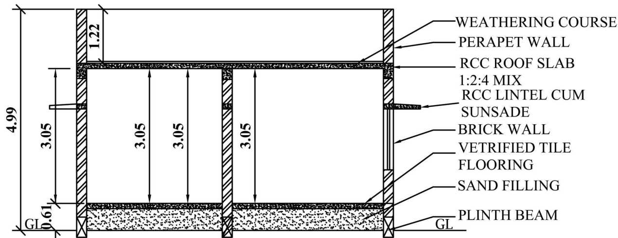
SECTION-AA
