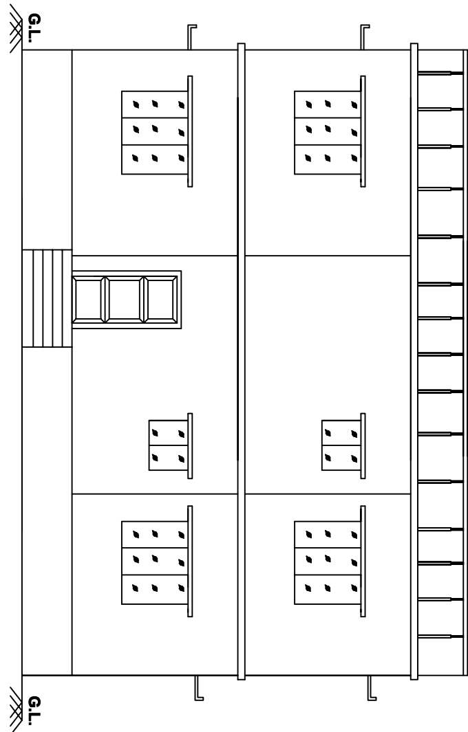
FRONT ELEVATION
