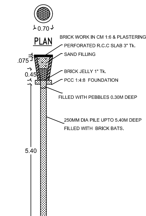
RAINWATER PERCOLATION PIT
