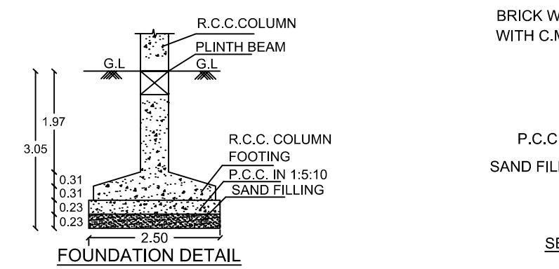
FOUNDATION DETAIL (DETAIL - B)
