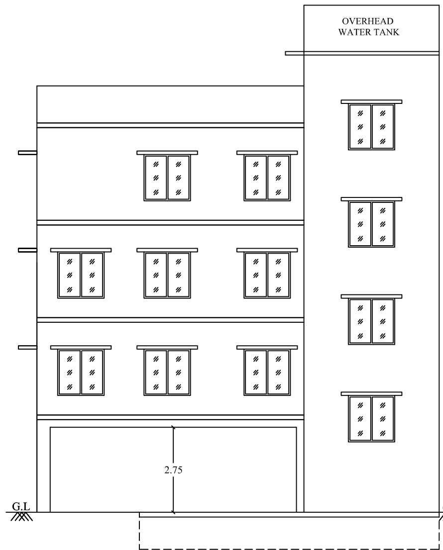
FRONT ELEVATION
