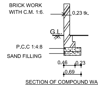
SECTION OF COMPOUND WALL
