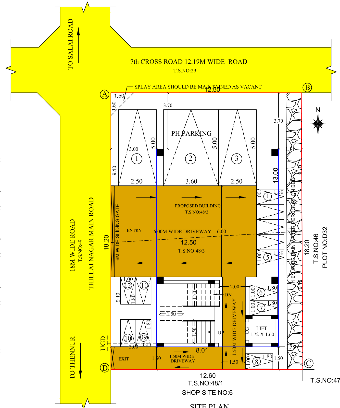
SITE PLAN
