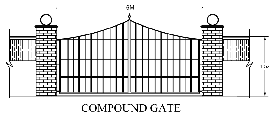
COMPOUND GATE
