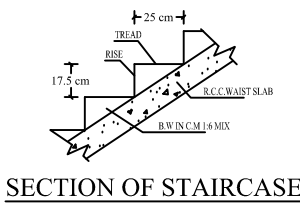
SECTION OF STAIRCASE
