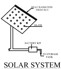
SOLAR SYSTEM
