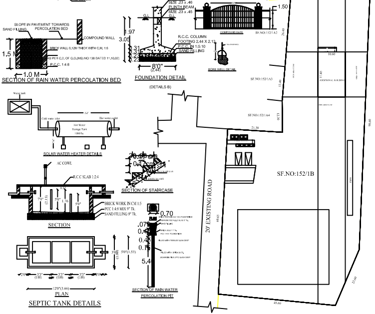
SCALE 1:800 SITE PLAN
