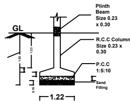
FOUNDATION DETAILS
