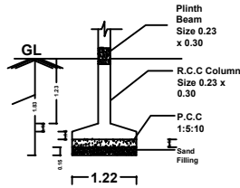
FOUNDATION DETAILS
