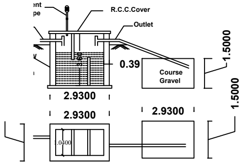
SEPTIC TANK & D-TRENCH DETAILS
