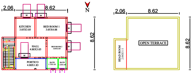
PROPO FLOOR
