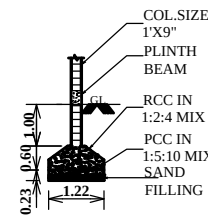
COLUMN DETAILS
