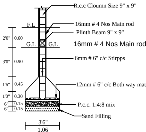
COLUMN DETIAL
