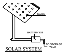
SOLAR SYSTEM
