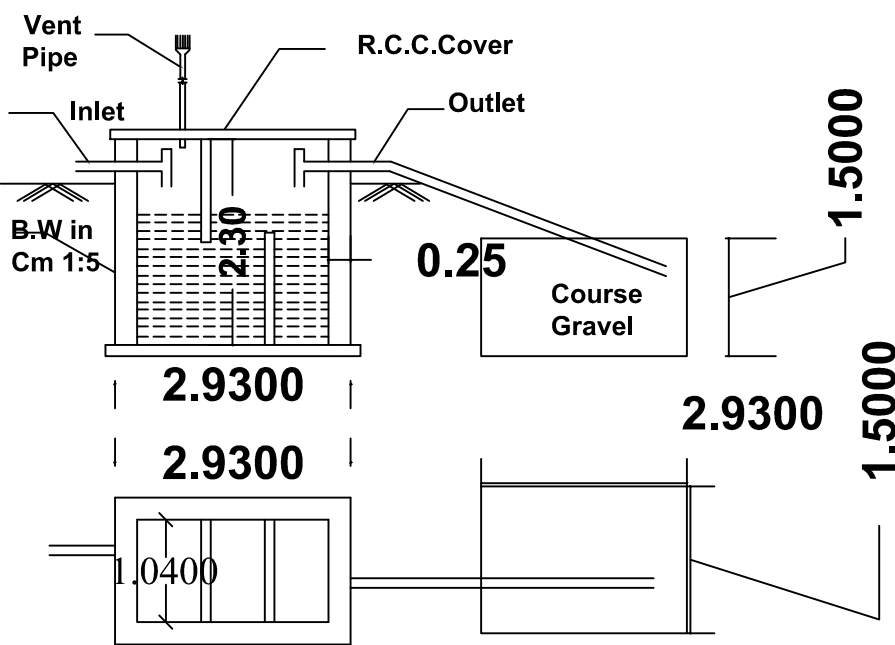
SEPTIC TANK & D-TRENCH DETAILS
