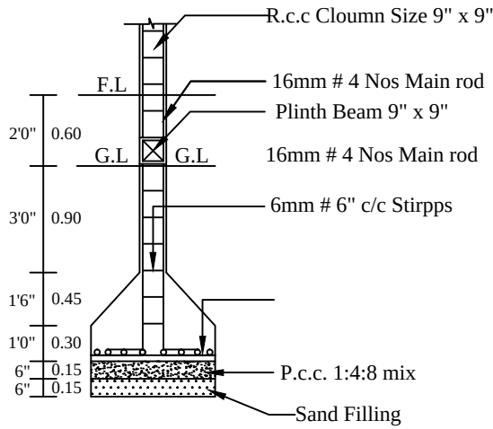
COLUMN DETIALS
