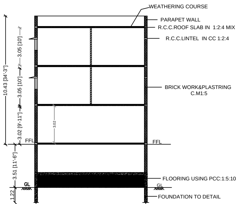
SECTION ON-XX
