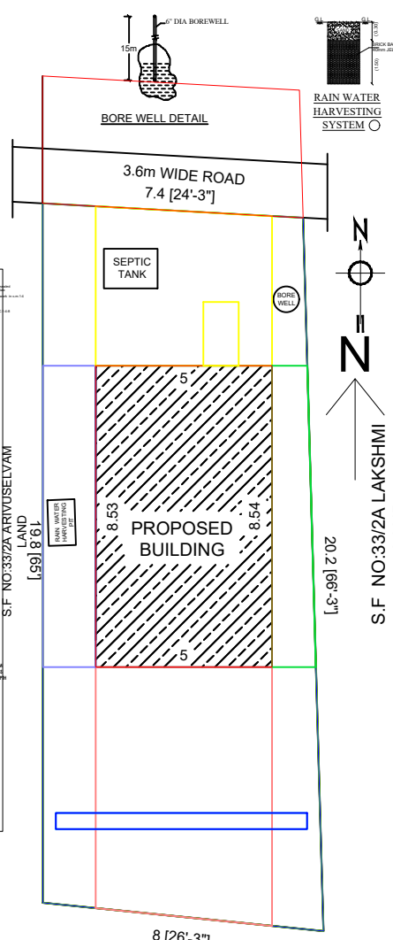
S.F. NO:33/2A LAKSHMI LAND SITE PLAN
