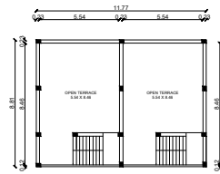
PROPOSED OPEN TERRACE FLOOR PLAN
