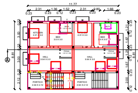
PROPOSED GROUND FLOOR PLAN
