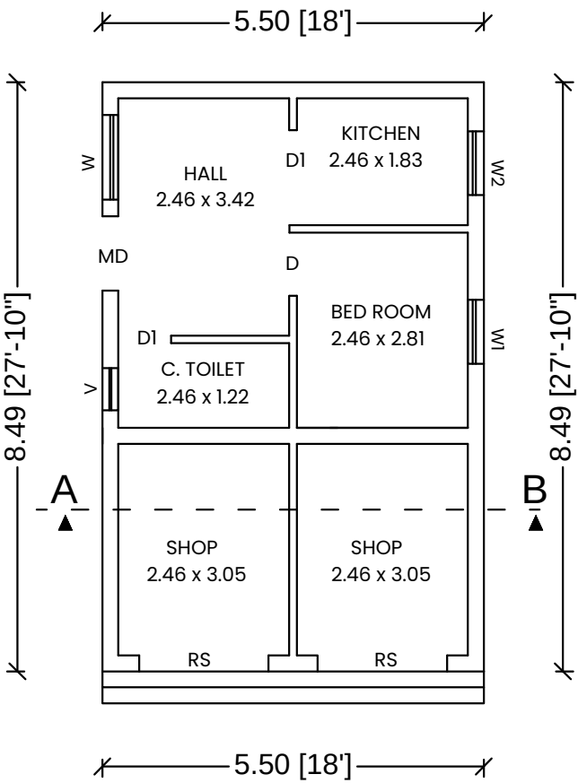
PLAN
