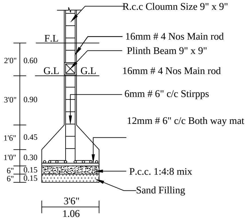
COLUMN DETIALS
