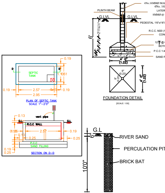
PERCOLATION PIT
