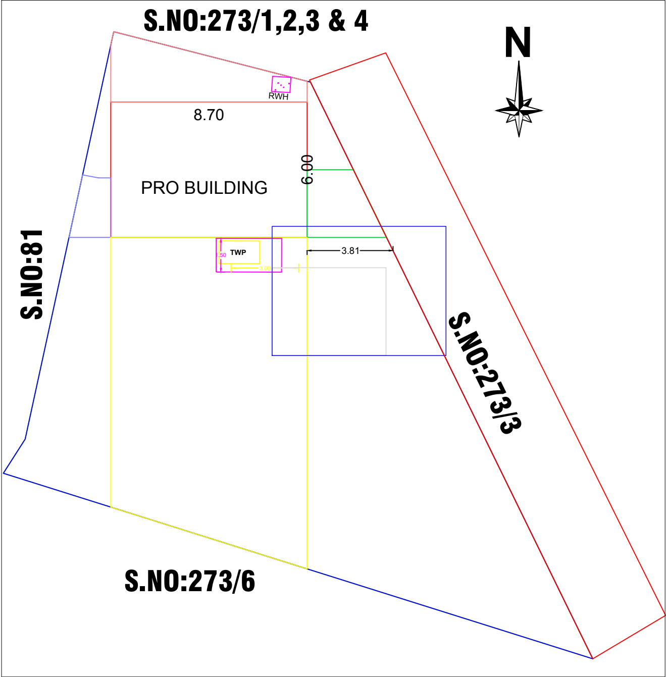
SITE PLAN
