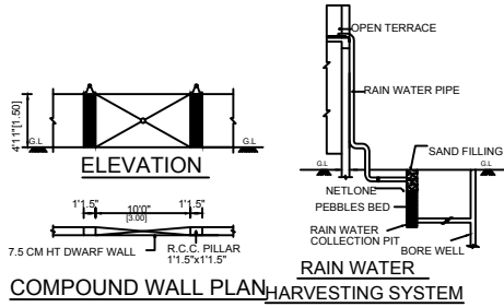
COMPOUND WALL PLAN,RAIN WATER HARVESTING SYSTEM
