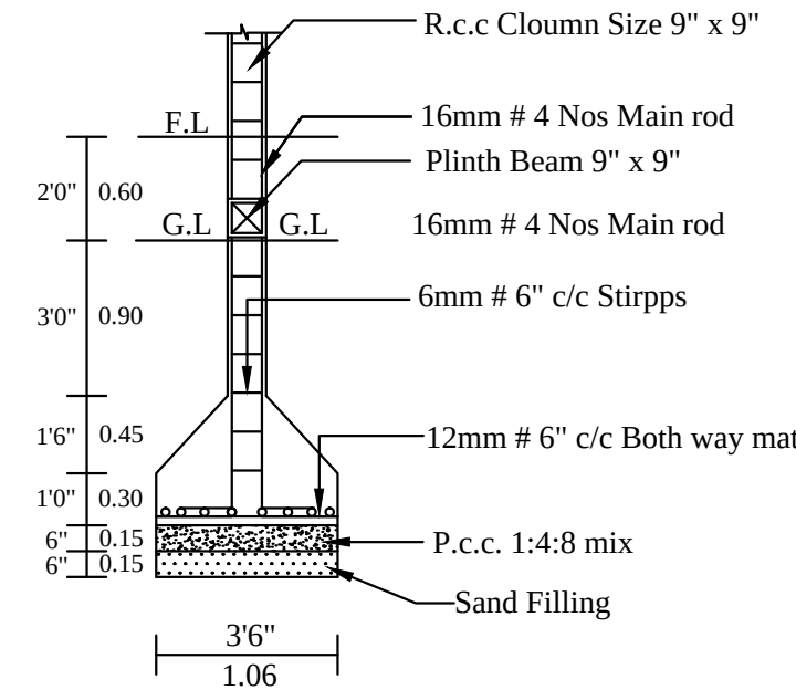
COLUMN DETAILS
