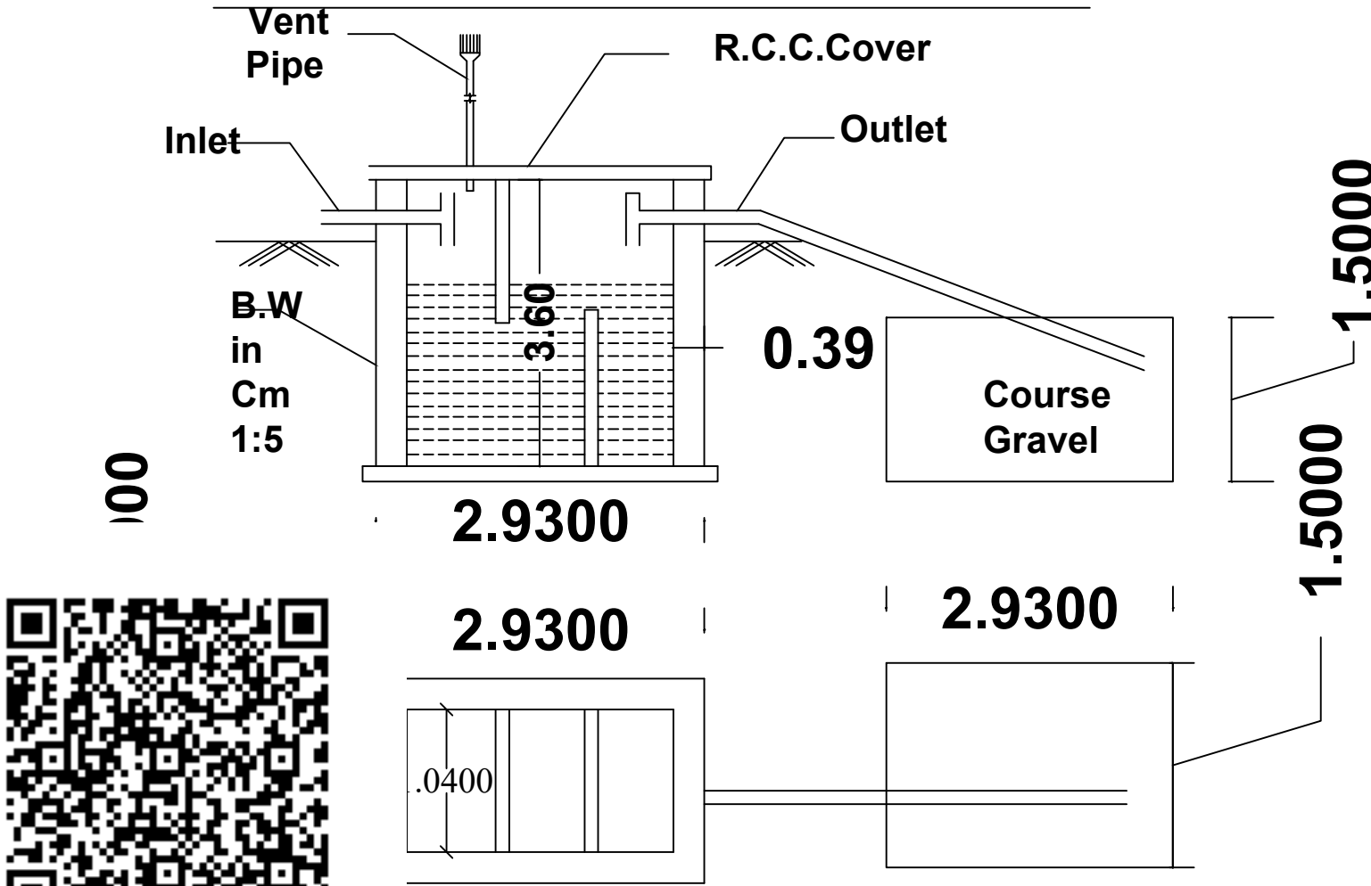
TANK & D-TRENCH DETAILS
