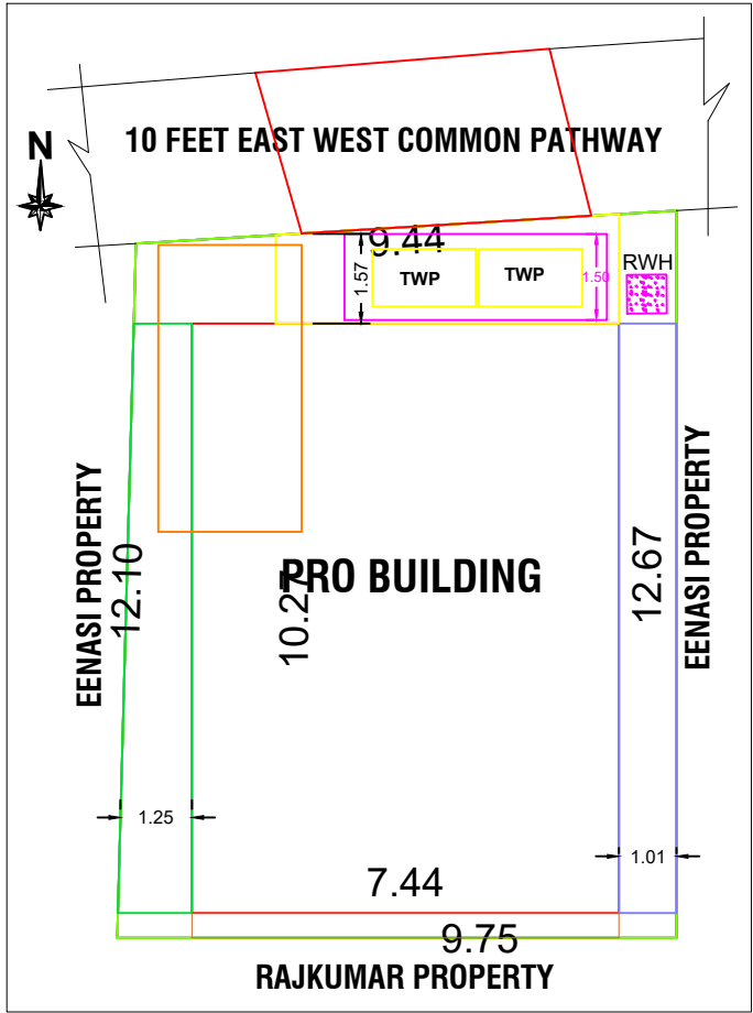
SITE PLAN
