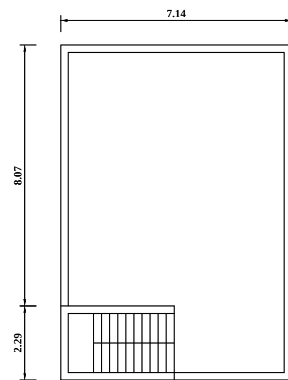
GROUND FLOOR ROOF PLAN
