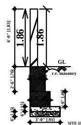
COMPOUND WALL
