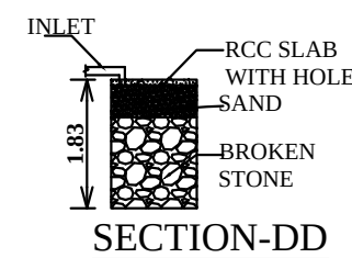
SECTION-DD
