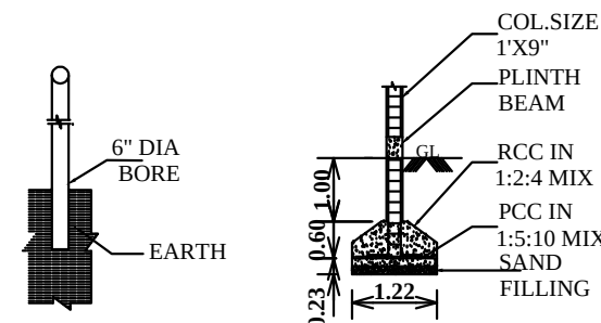
BORE WELL
