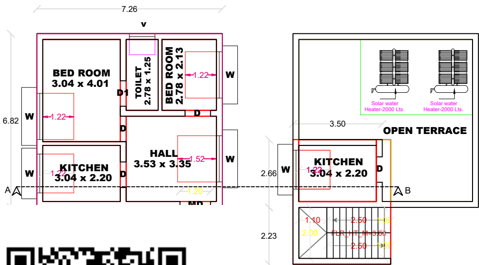
FIRST FLOOR PLAN OPEN TERRACE PLAN
