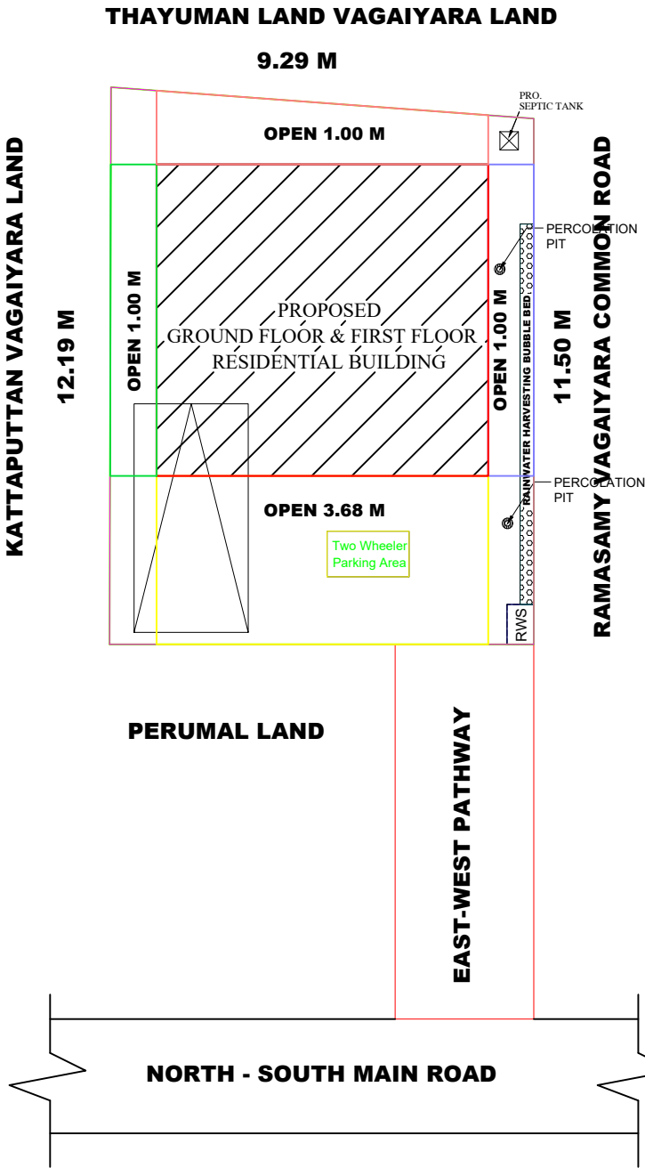
SITE PLAN (SCALE 1:1)
