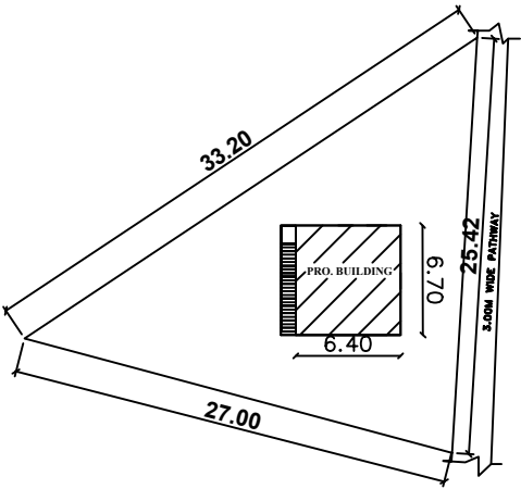
SITE PLAN
