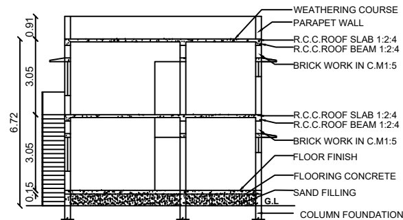
SECTION ON SS
