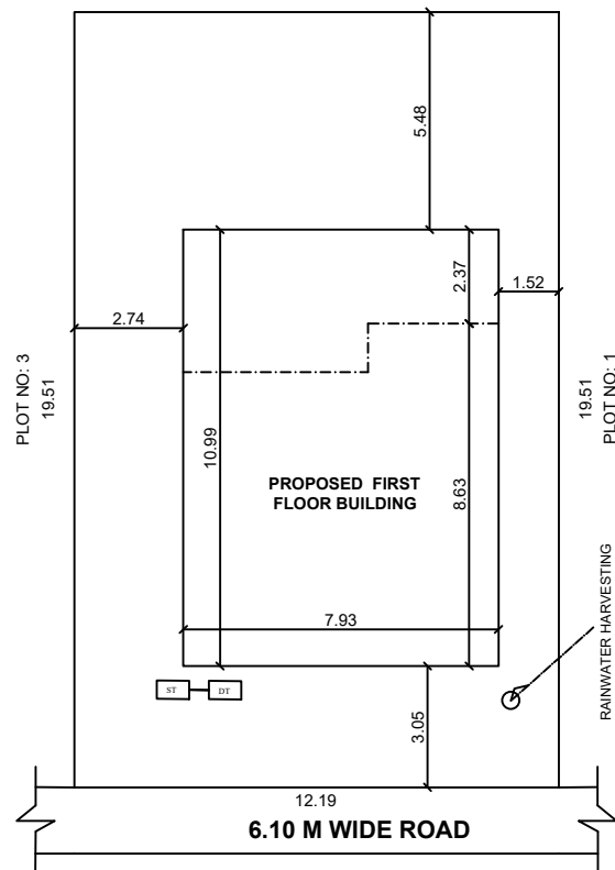
SITE PLAN
