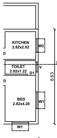
FIRST FLOOR PLAN (PRO)
