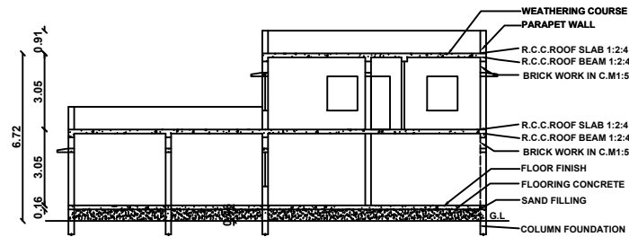
SECTION ON GG
