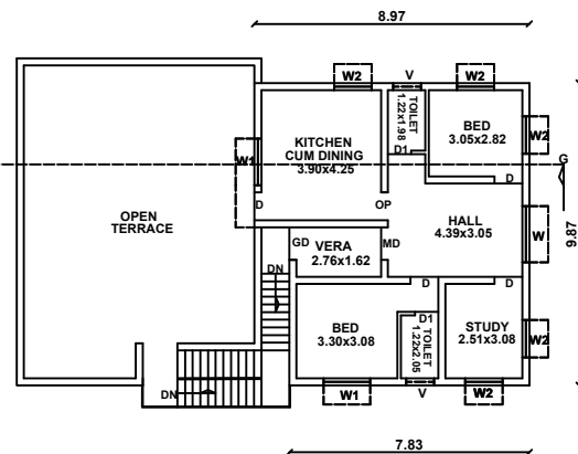
FIRST FLOOR PLAN (PRO)
