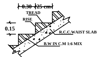
SECTION OF STAIRCASE
