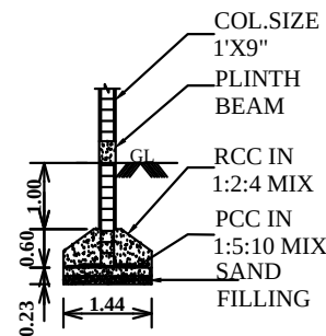
COLUMN DETAILS
