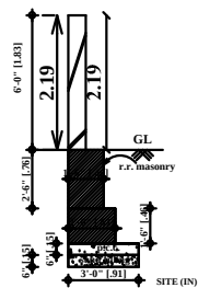
COMPOUND WALL
