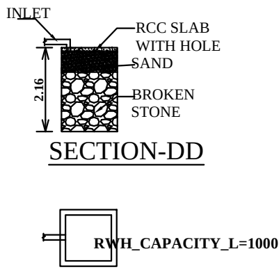
PLAN OF RWH
