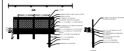
COMPOUND WALL RADIATION SUN DETAIL
