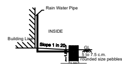
RAINWATER HARVESTING
