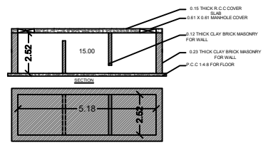
SEPTIC TANK & DISPERSION TRENCH DETAILS
