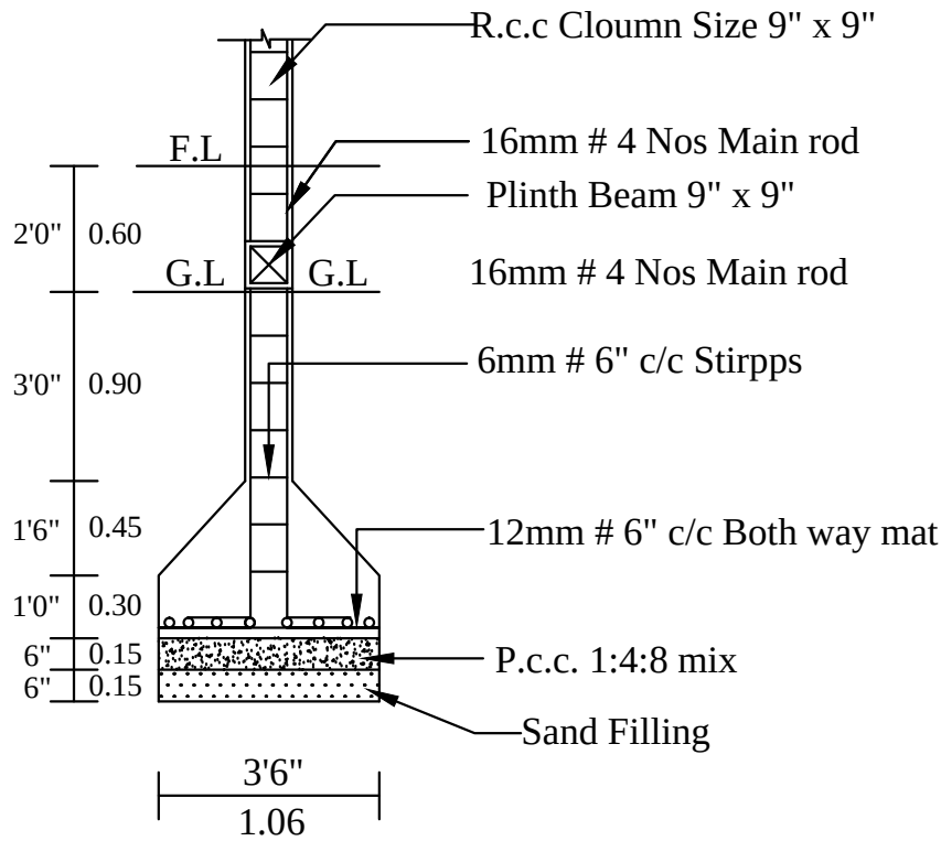
COLUMN DETIALS
