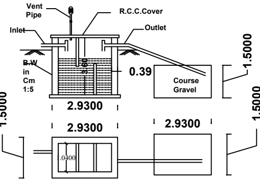
SEPTIC TANK & D-TRENCH DETAILS
