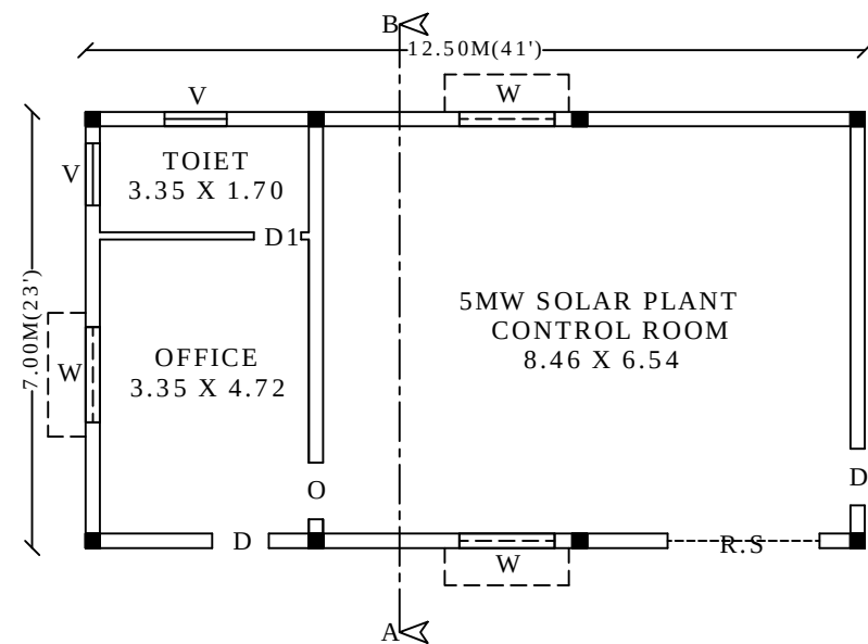
PRO.GROUND FLOOR PLAN (NORTH FACING)
