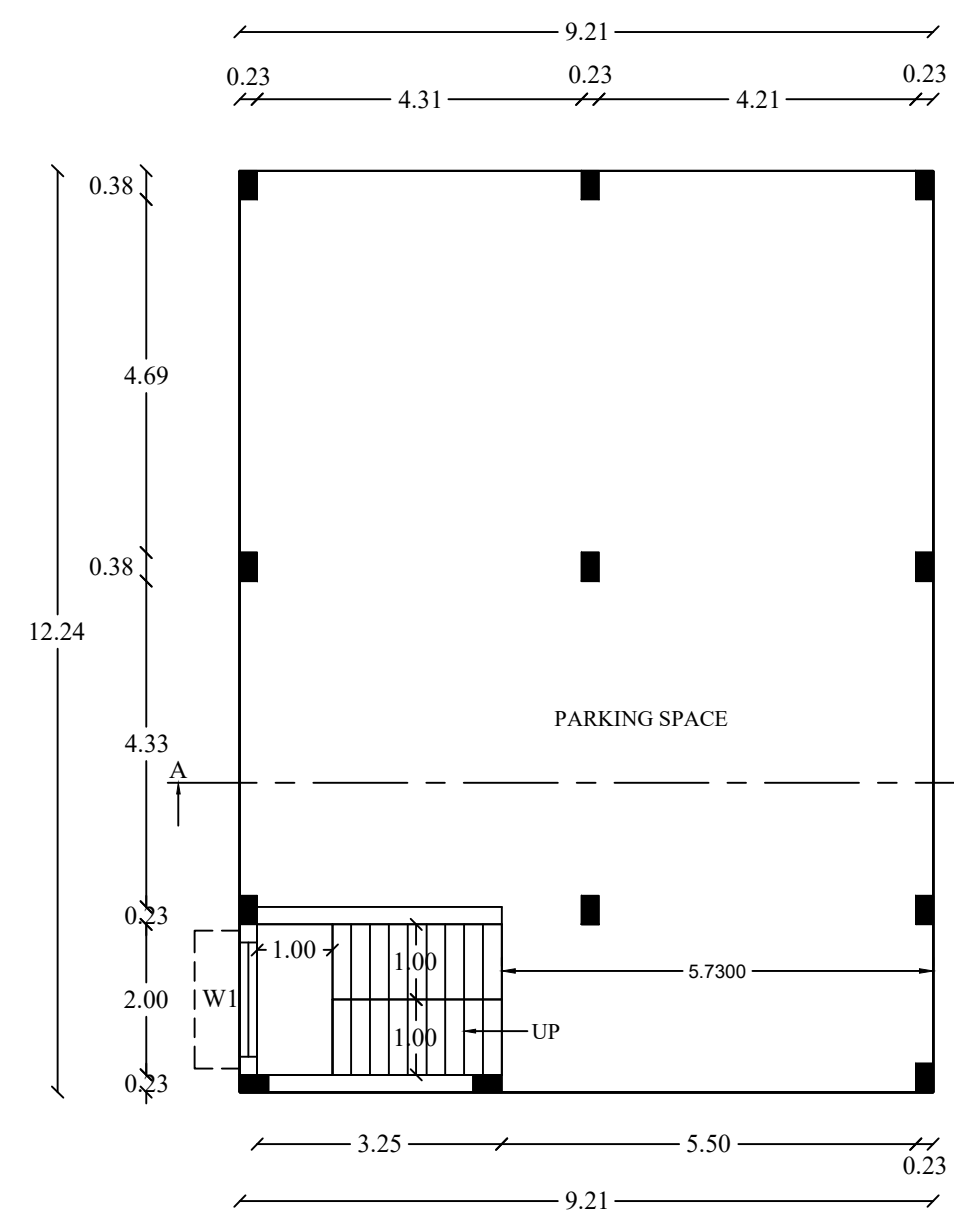
STILT FLOOR PLAN (PARKING)
