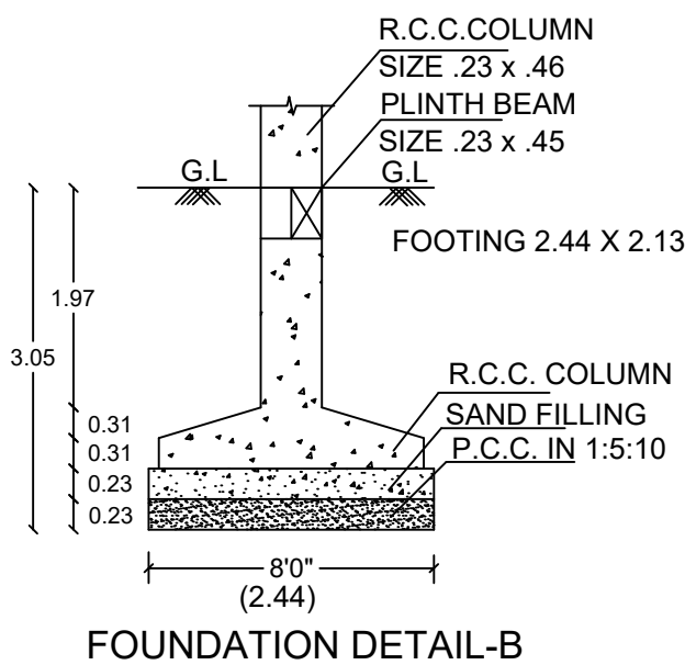
FOUNDATION DETAIL-B
