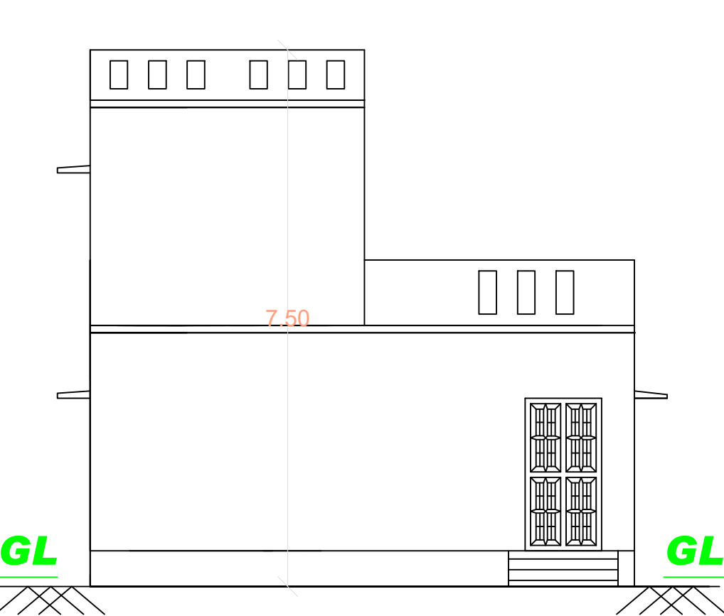
FRONT ELEVATION
