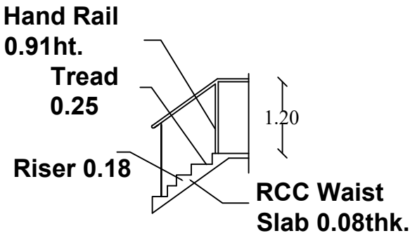
STAIRCASE DETAILS
