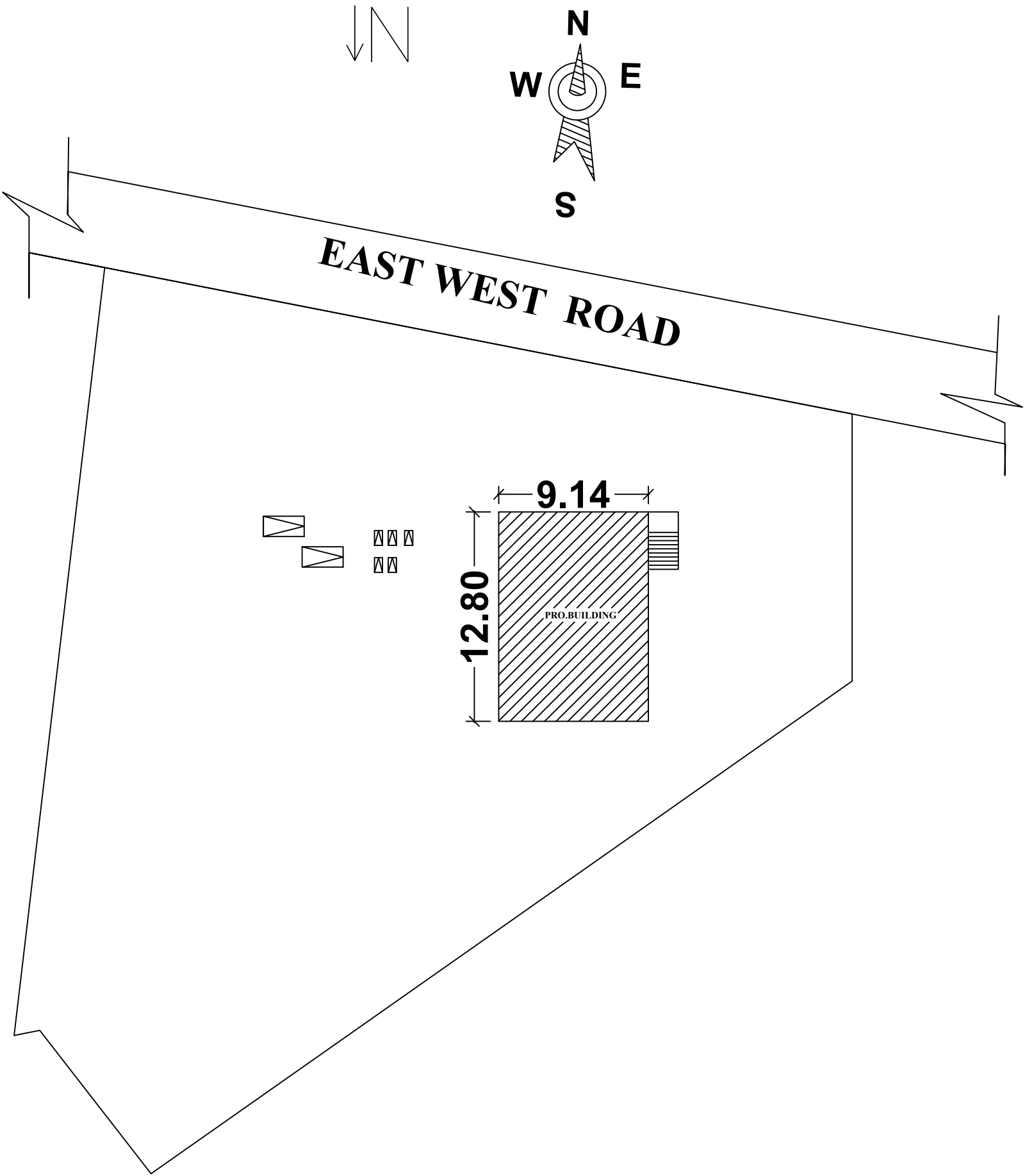
SITE PLAN
