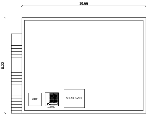
PRO GROUND FLOOR ROOF PLAN
