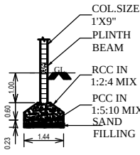
COLUMN DETAILS
