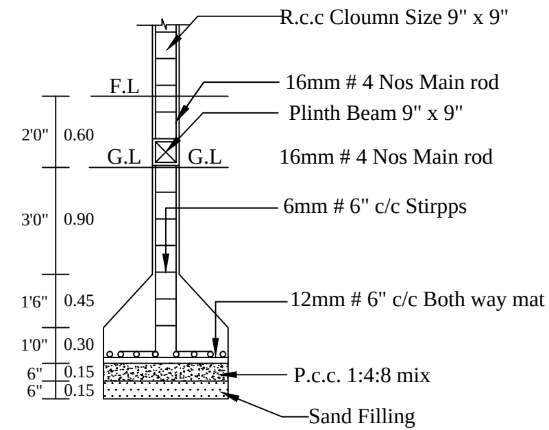
COLUMN DETAILS
