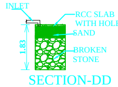
SECTION-DD
