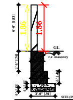
COMPOUND WALL
