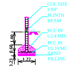
COLUMN DETAILS
