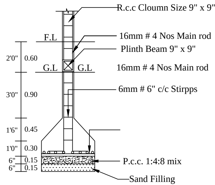
COLUMN DETIALS
