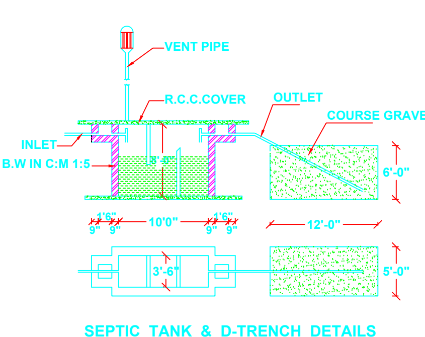
SEPTIC TANK & D-TRENCH DETAILS (NOT TO SCALE)
