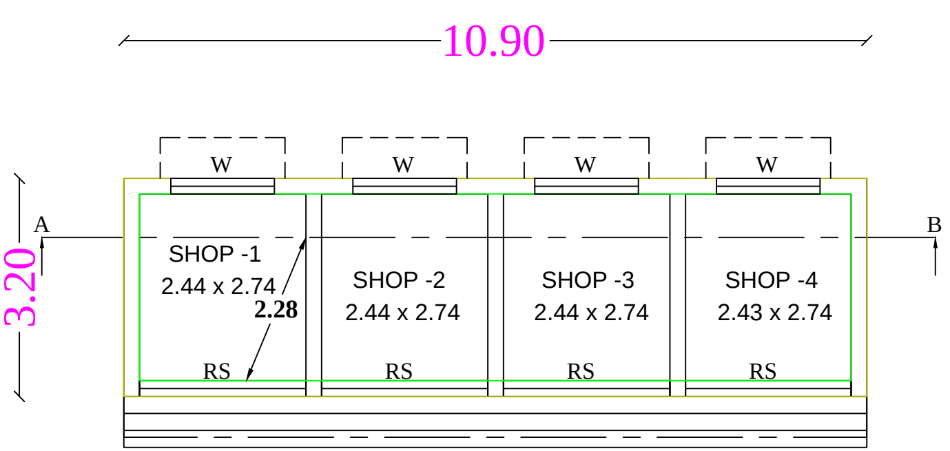
GROUND FLOOR PLAN (PROPOSED)
